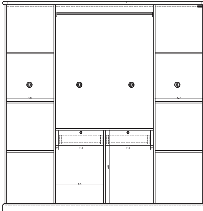
4 DOOR INNER VIEW
